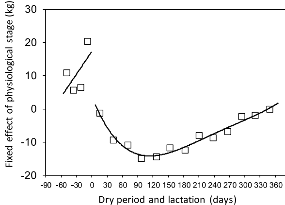
Effect physiological stage (model HG BG HW)
