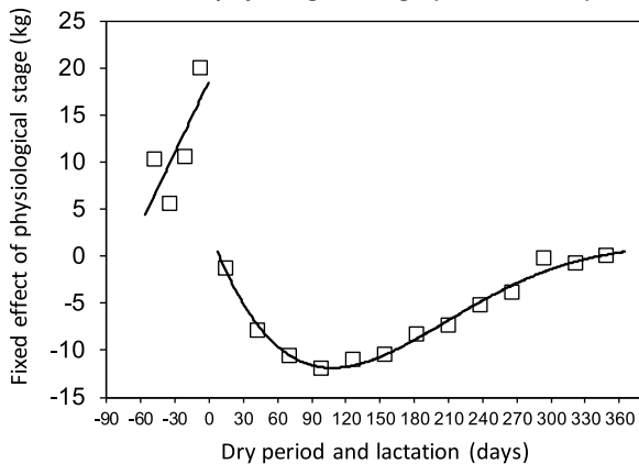
Effect physiological stage (model HG BG)
