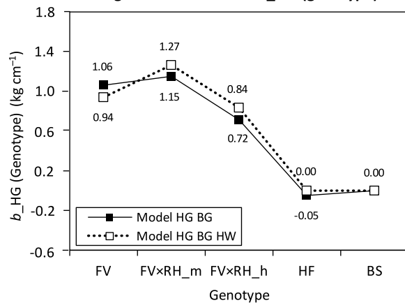
Regression coefficient b_{HG} (genotype)
