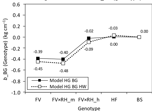
Regression coefficient b_{BG} (genotype)
