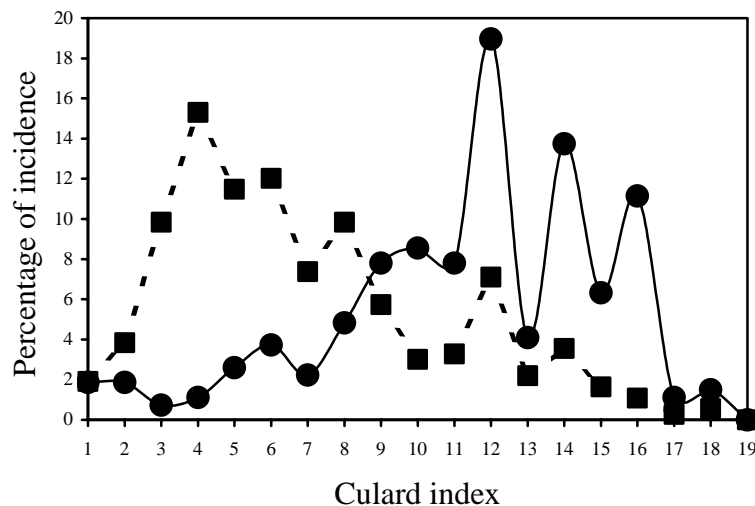
Fig. 2: Frequency of Culard index score (in percentage) by parents' muscularity score. (■) Class 0 sires' offspring. (●) Class 2 dams' offspring
