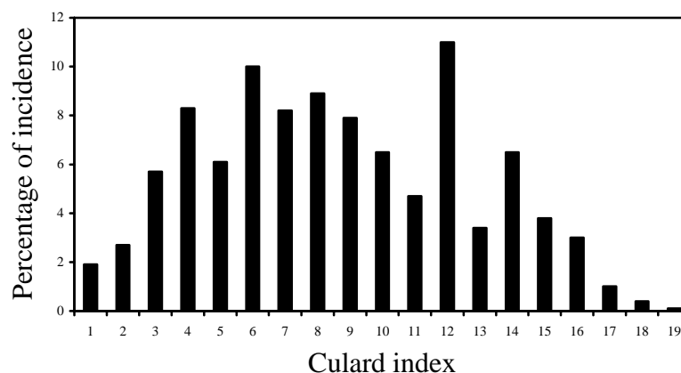
Fig. 1: Frequency of culard index score (in percentage) in the analysed database
